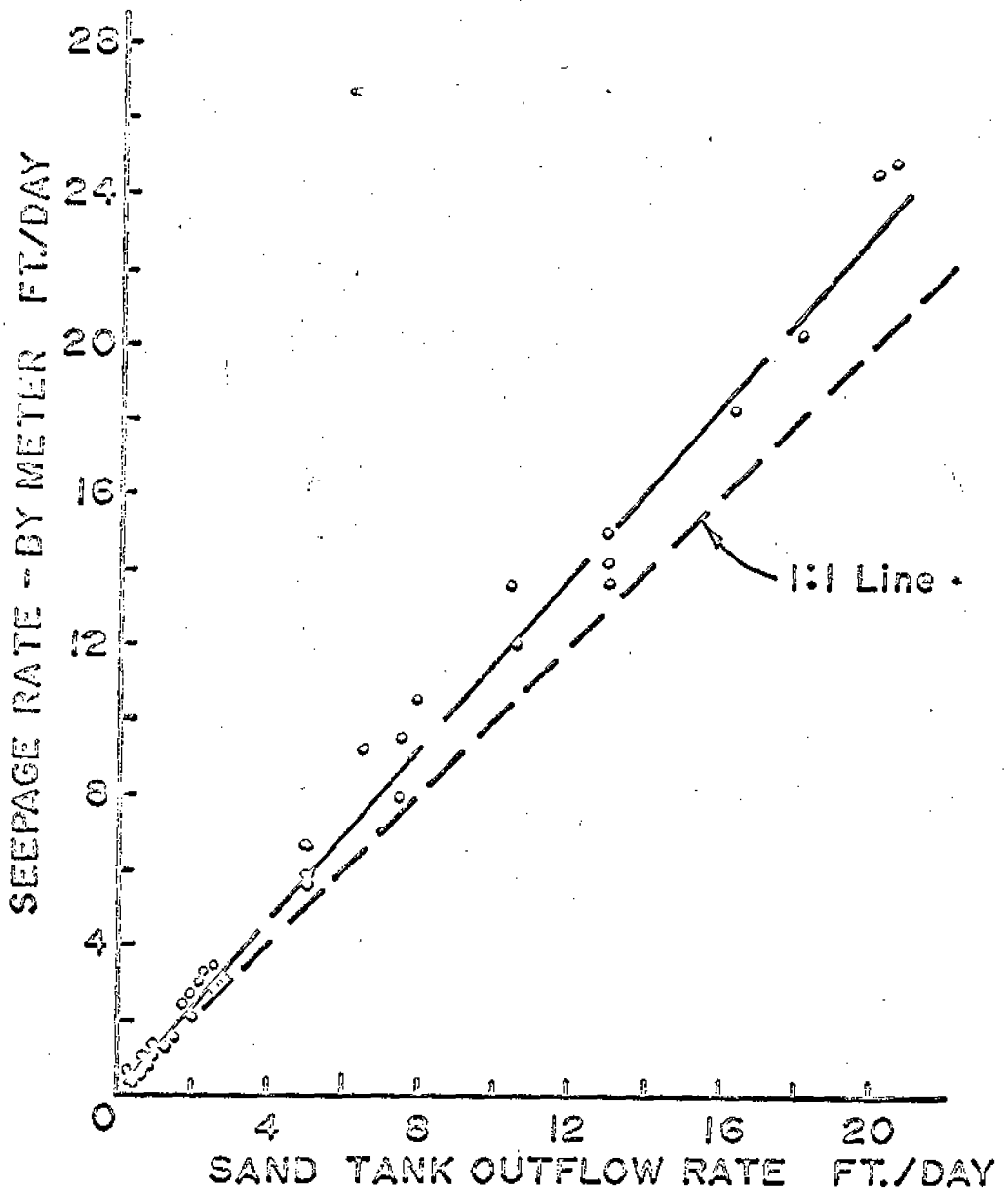
Figure 4. Comparison of sand tank outflow rates and seepage meter measurements.
