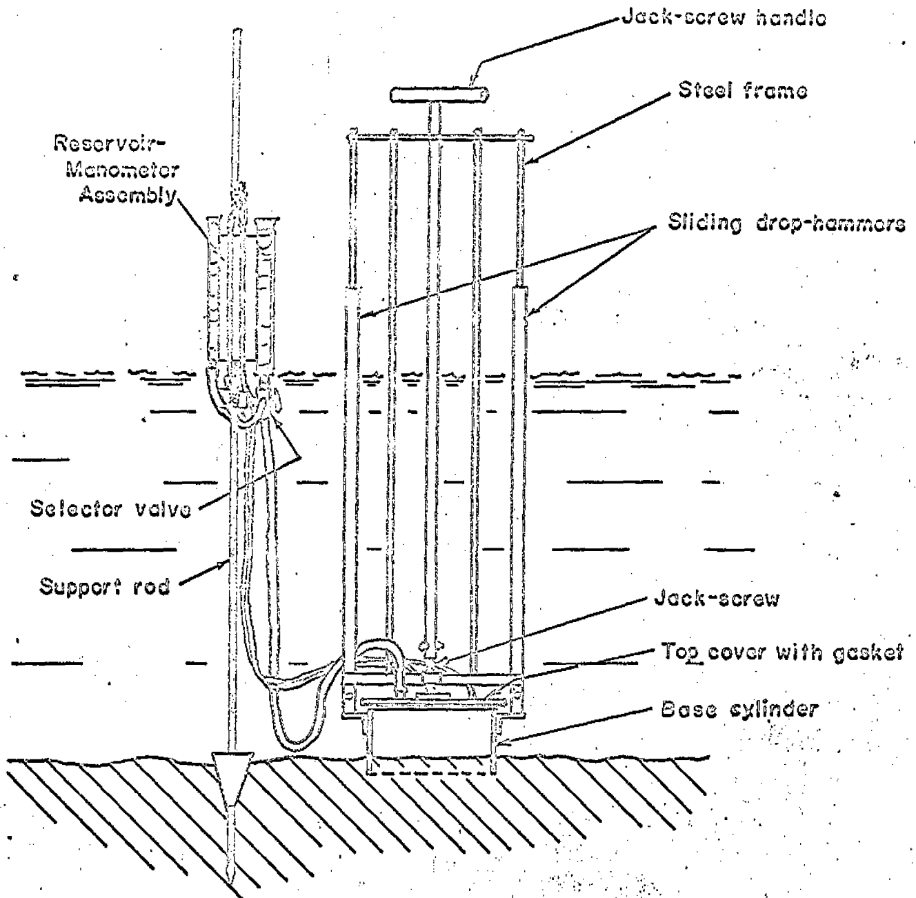
Figure 1. Overall view of seepage meter equipment
