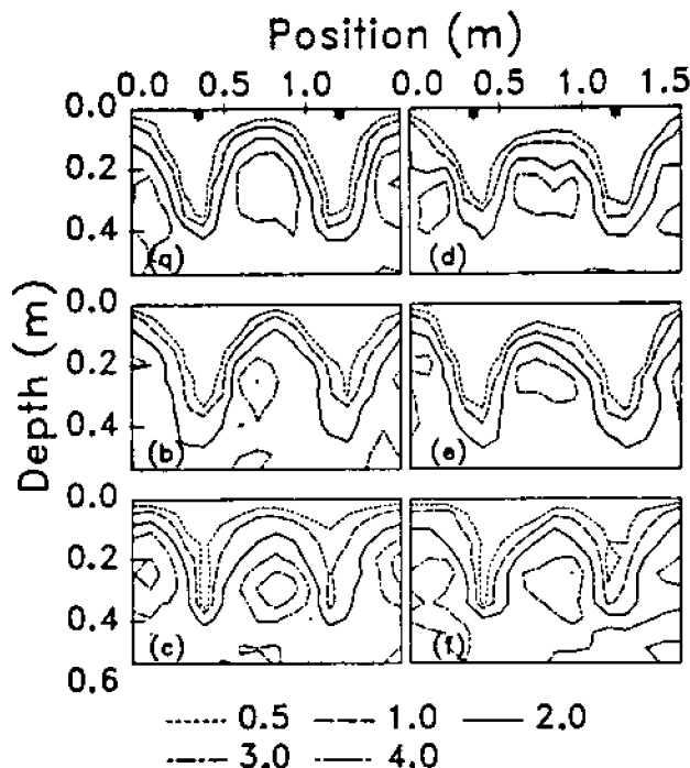
Fig. 1. Cross sectional view of the soil strength patterns for SS (a), PT (b), and KE (c) of the minimum surface tillage treatment and the SS (d), PT (e), and KE (f) of the conventional surface tillage treatment for April 1985. Each diagram is the average of four replicates. The asterisks show the positions of the rows.
