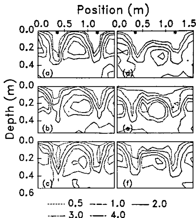
Fig. 2. Cross sectional view of the soil strength patterns for SS (a), PT (b), and KE (c) of the minimum surface tillage treatments and the SS (d), PT (e), and KE (f) of the conventional surface tillage treatment for April 1986. Each diagram is the average of four replicates. The asterisks show the positions of the rows.
