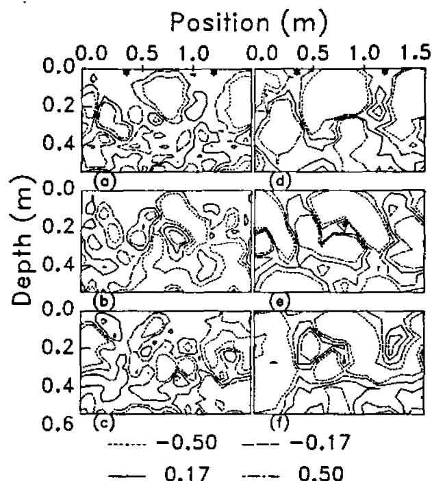
Fig. 3. Cross sectional view of the difference (conventional minus minimum surface tillage treatment) of the soil strength patterns for SS (a), PT (b), and KE (c) in April 1985 and the SS (d), PT (e), and KE (f) April 1986. Each diagram is the average of four replicates. The asterisks show the positions of the rows.
