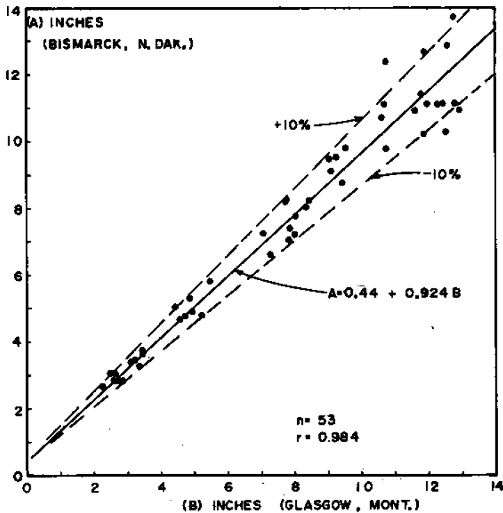
FIG. 8.—COMPARISON OF INDIVIDUAL MONTHLY VALUES OF SOLAR RADIATION AT TWO LOCATIONS APPROXIMATELY 300 MILES APART
