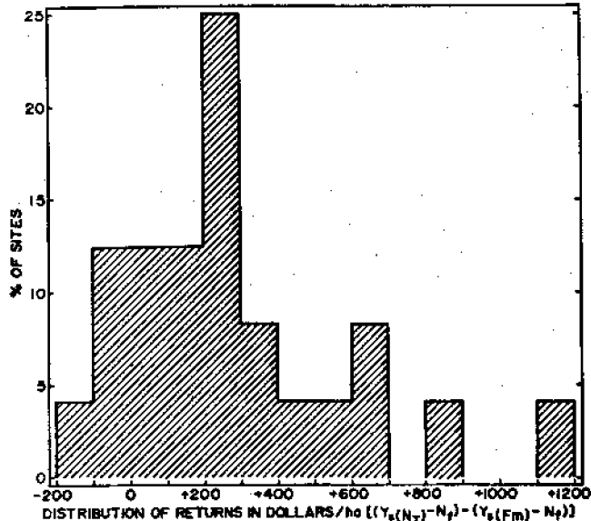
Fig. 5. Frequency distribution of the difference in increased returns from sucrose production when using N fertilizer recommendations based on a soil test ( N_T ) as compared to those made by fieldmen ( F_M ) on 24 sites in 1971 ( Y_s = sucrose yield at $0.55/kg, N_T = N fertilizer at $0.66/kg).
