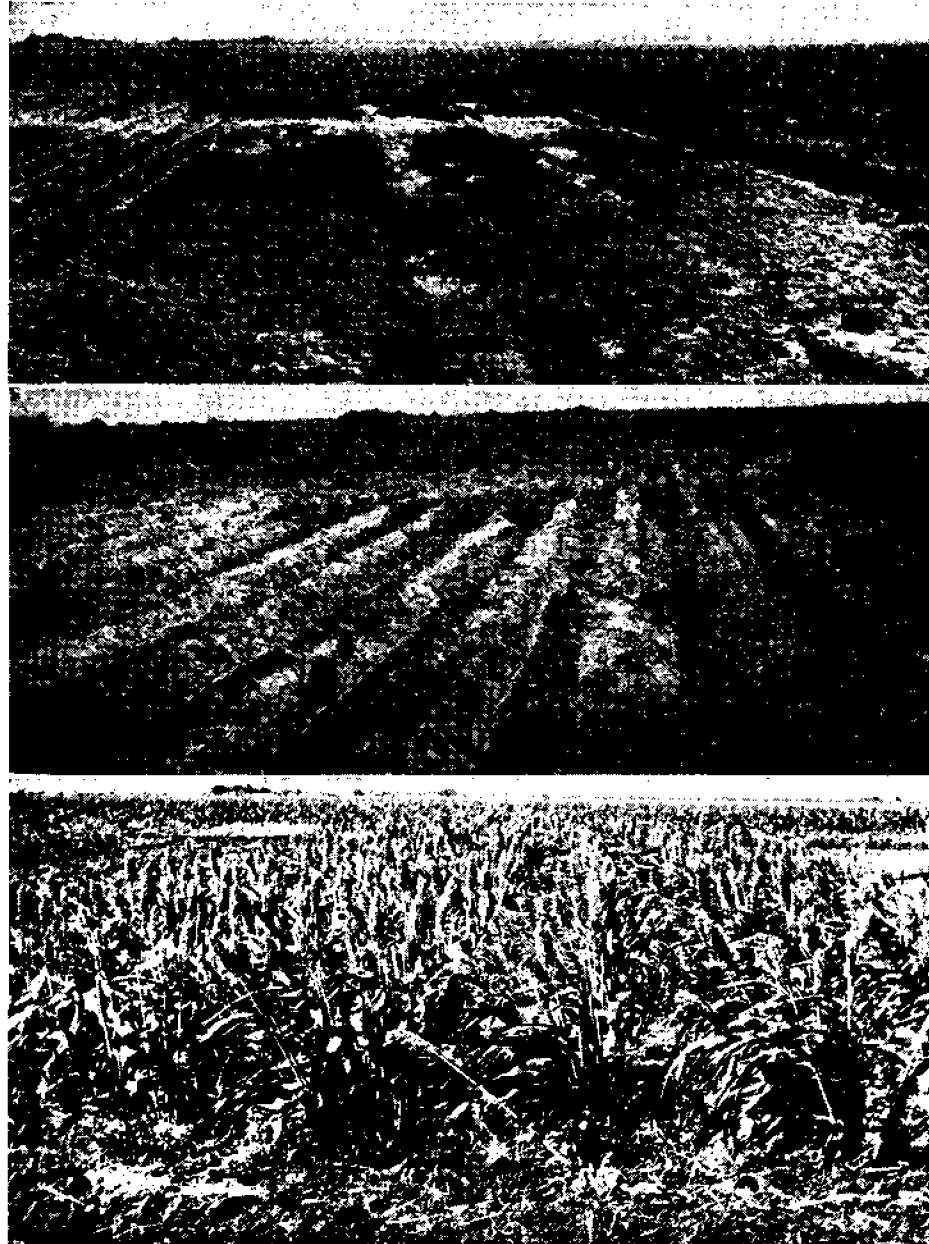
Typical experimental plots under the three different treatments on highly saline soil as they appeared in June 1964. Grain sorghum was planted on all the plots in February 1964. (Top) Conventionally tilled plots produced only a few salt tolerant weeds. (Center) Permanent ridge-furrow plots presented serious problems of weed control and produced no grain. (Bottom) Cotton bur mulched plots produced a good crop of sorghum.
