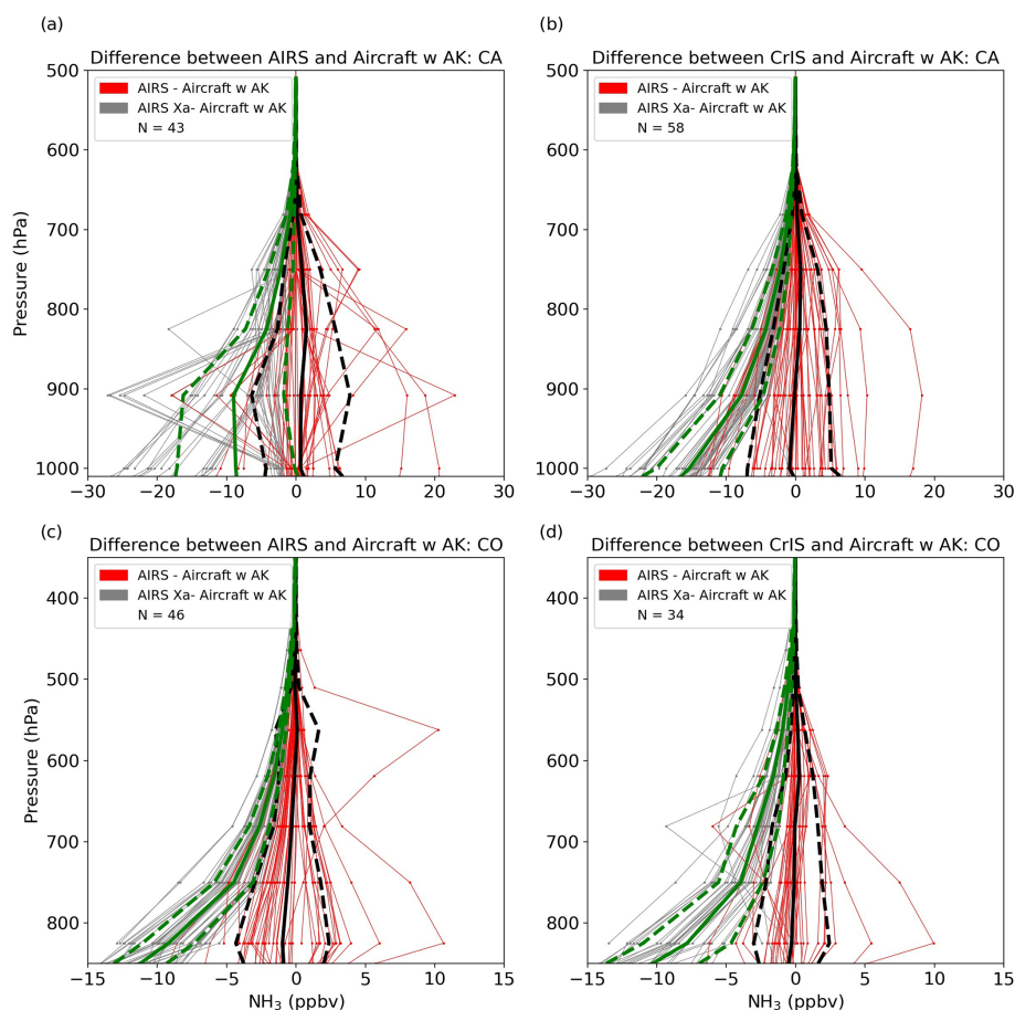
Figure 5. Difference between AIRS and aircraft NH 3 profiles ( a , c ) and CrIS and aircraft ( b , d ) during DISCOVER-AQ in California ( a , b ) and Colorado ( c , d ). The averaging kernel has been applied to the aircraft data; red lines show differences between the retrieved profiles and the aircraft data, solid black lines indicate mean bias and dashed black lines standard deviations; gray lines show differences between the a priori profiles and the aircraft, solid green lines indicate mean bias and dashed green lines standard deviations.
