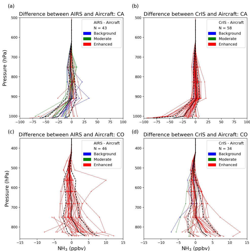
Figure 3. Difference between AIRS and aircraft NH 3 profiles ( a , c ) and CrIS and aircraft ( b , d ) during DISCOVER-AQ in California ( a , b ) and Colorado ( c , d ); solid line indicates mean bias and dashed lines standard deviations. Colors indicate choice of a priori profile.
