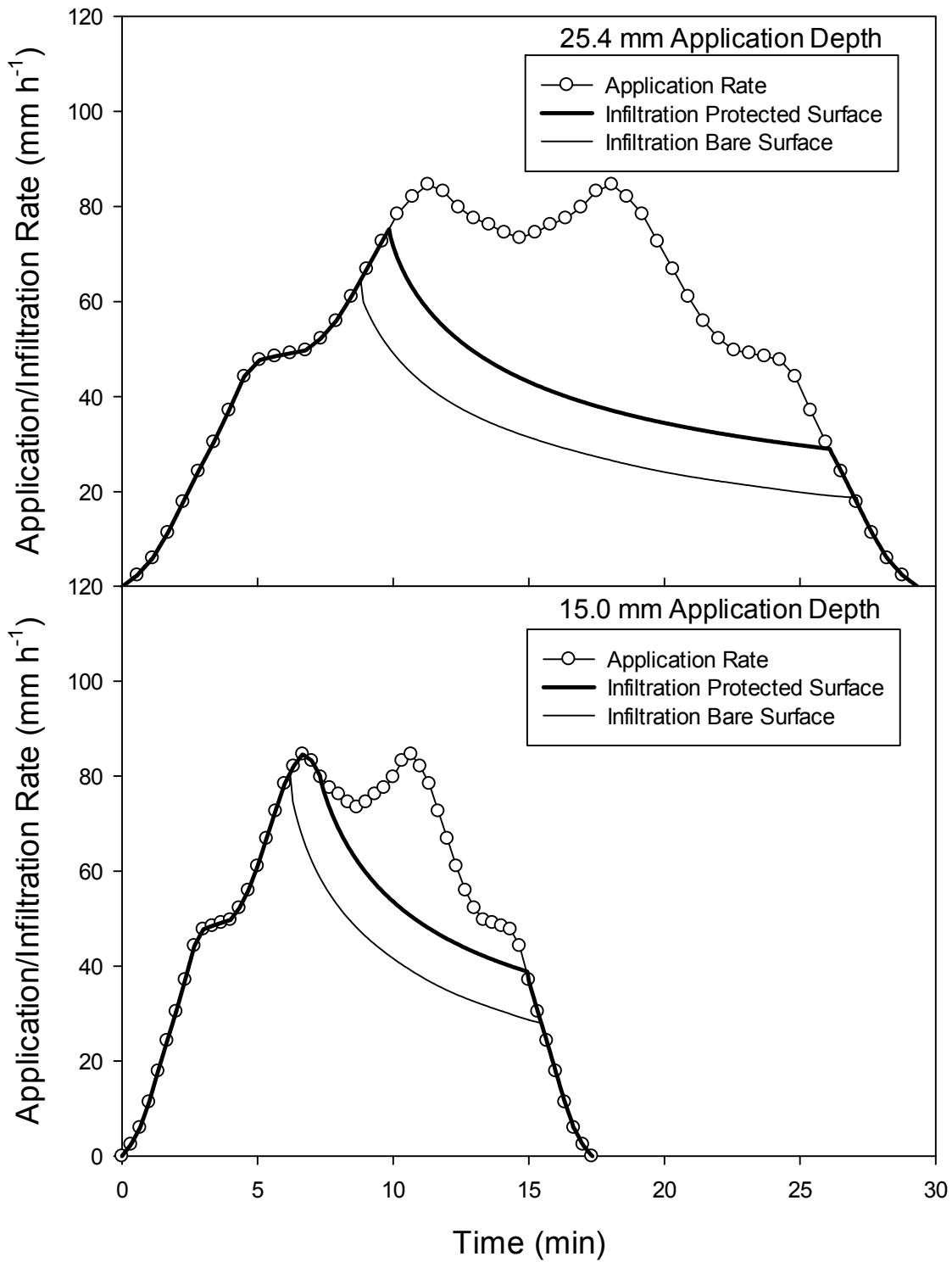
Figure 7. Model predicted infiltration rate for the Atwood silty clay loam soil under center pivot irrigation with the R3000 red plate sprinkler for protected and bare soil surface conditions and application depths of 25.4 and 15.0 mm.
