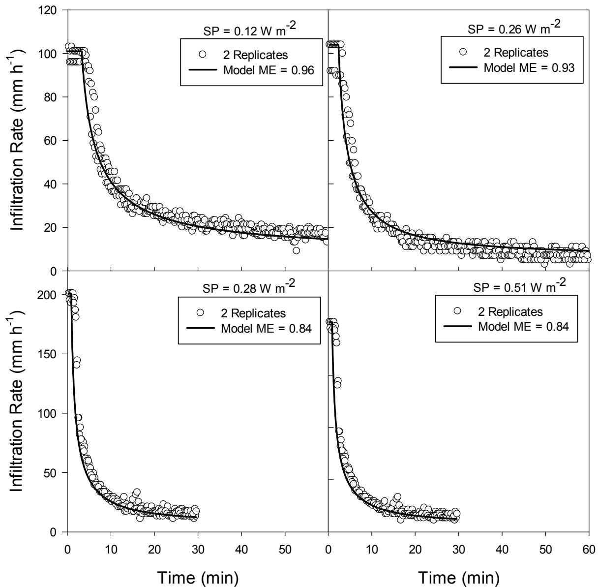
Figure 5. Infiltration model fit to measured infiltration for Walla Walla silt loam soil at four levels of specific power applied by laboratory simulated rainfall.
