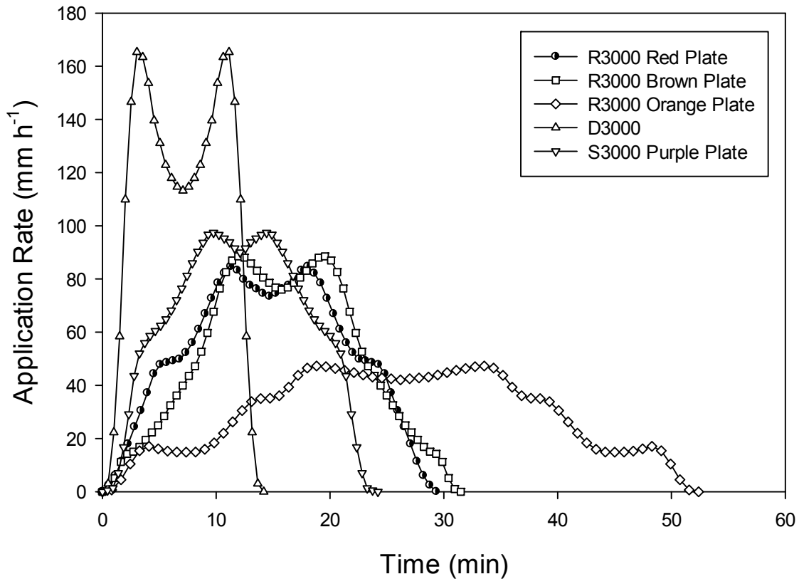
Figure 1. Average composite application rate profile for five sprinklers used in this study spaced 3m along a center pivot lateral.
