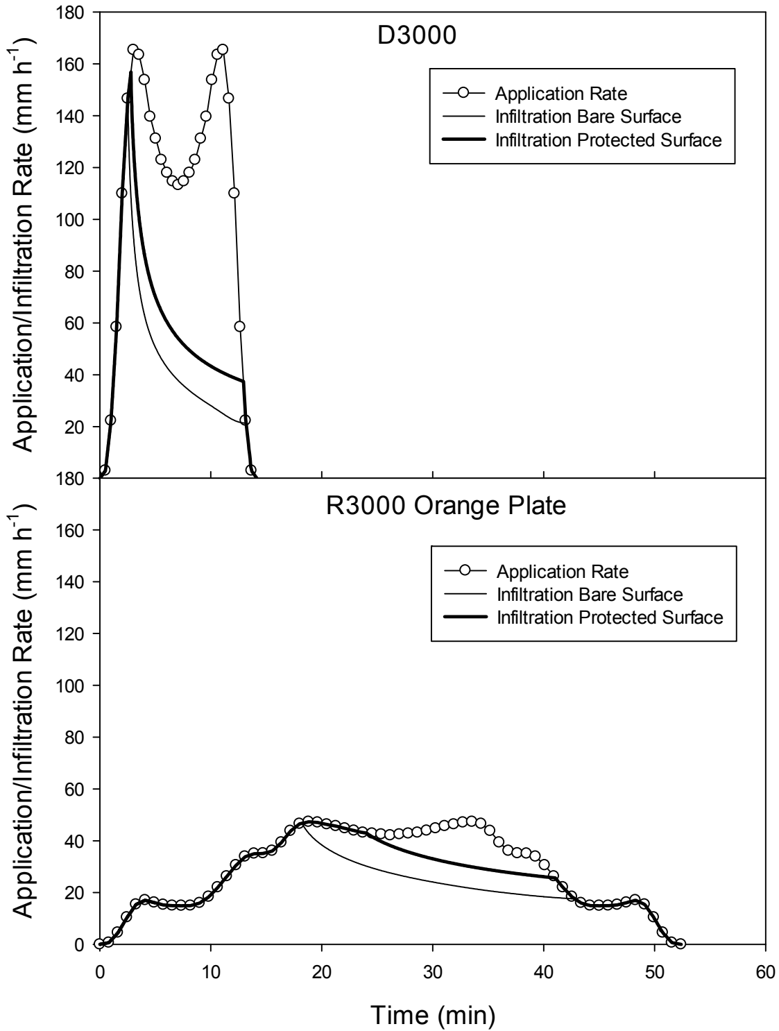
Figure 8. Model predicted infiltration rate for the Atwood silty clay loam soil under center pivot irrigation with the D3000 and R3000 orange plate sprinkler for protected and bare soil surface conditions and an application depth of 25.4 mm.
