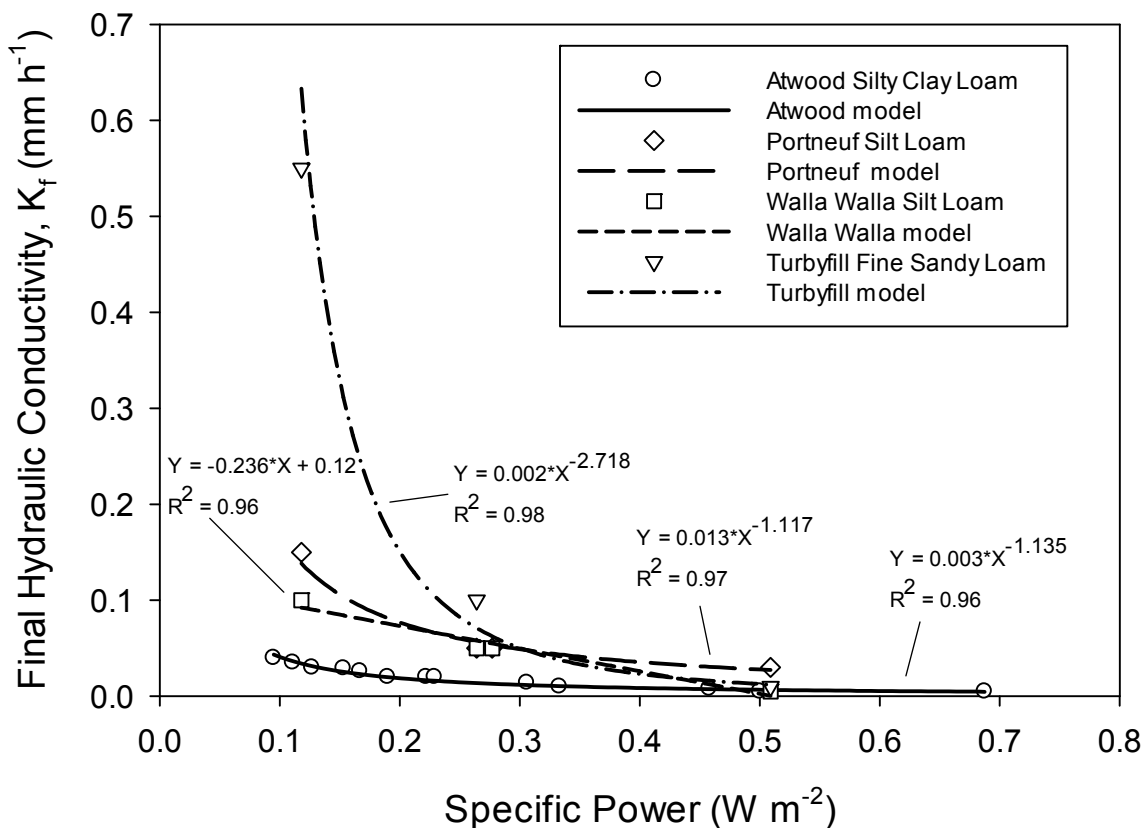
Figure 6. Relationship between final hydraulic conductivity of surface seal and specific power for each soil used to model infiltration under surface seal formation in this study.
