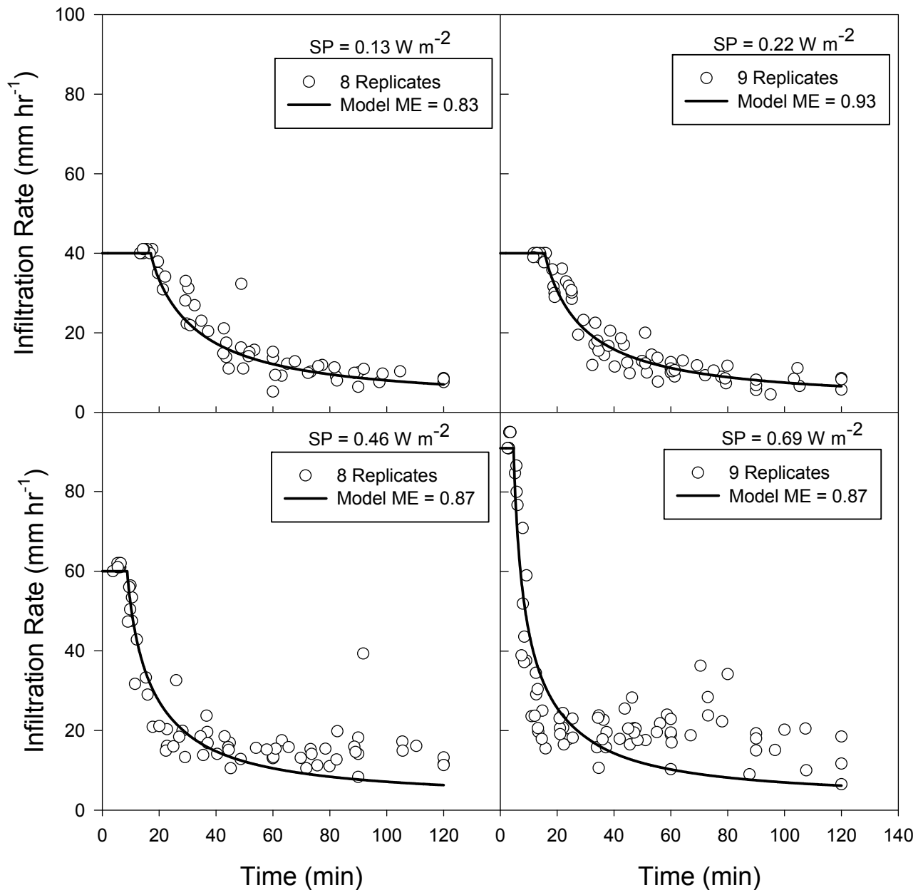
Figure 4. Infiltration model fit to measured infiltration from soil columns of Atwood silty clay loam soil reported by Baumhardt (1985) under four levels of specific power applied by simulated rainfall.
