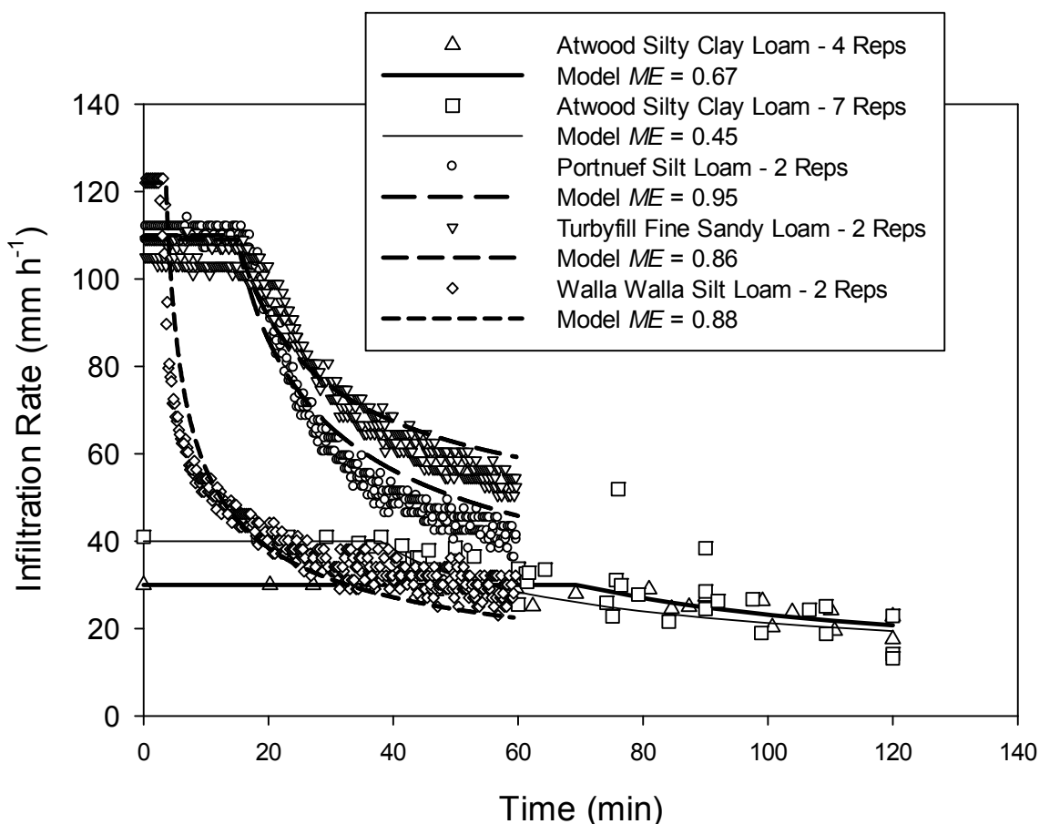
Figure 3. Model prediction of infiltration into each soil compared to measured infiltration under rainfall simulator when the soil surface was protected from droplet impact.
