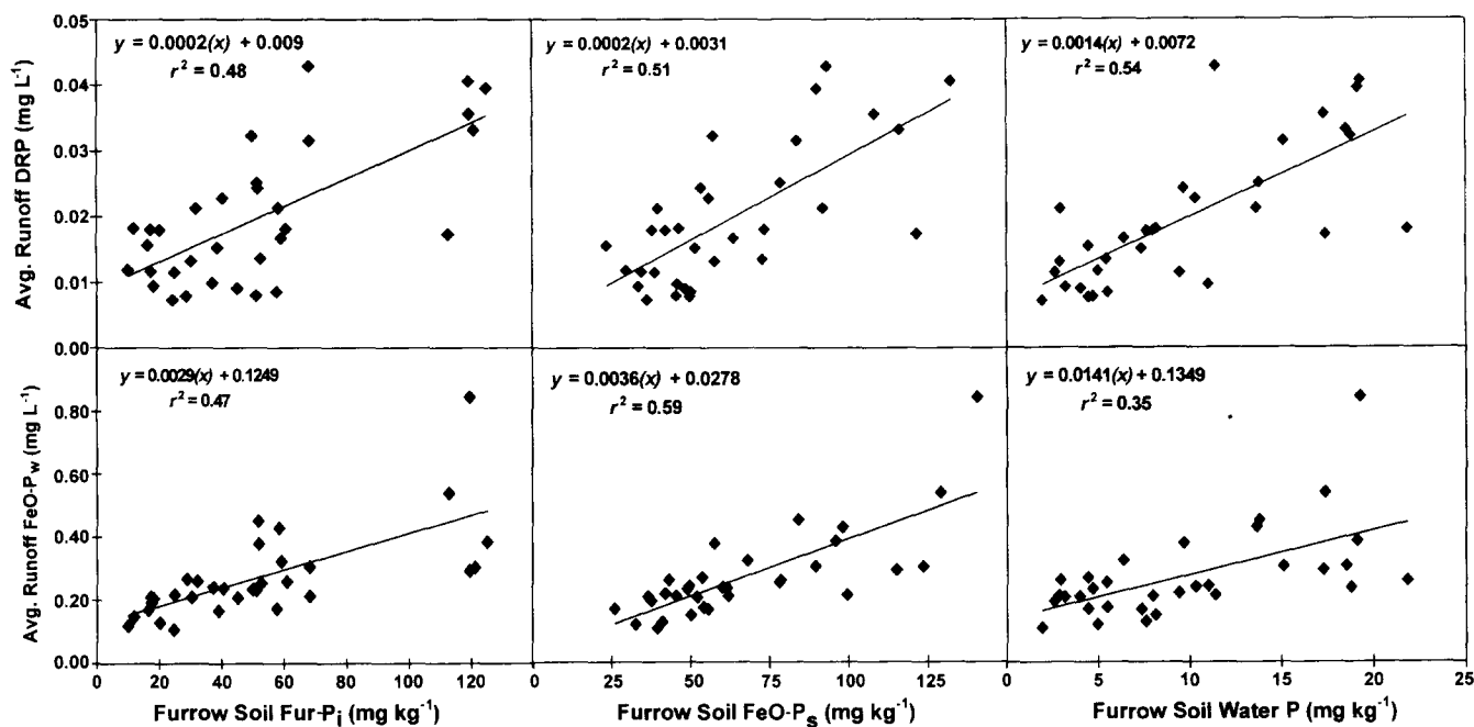
Fig. 1. Linear relationships between average runoff dissolved reactive phosphorus (DRP) and iron-oxide impregnated paper-extractable phosphorus from unfiltered runoff water (FeO-P w ) concentrations, and furrow soil P tests ( r^2 > 0.12 significant at 5% probability).
