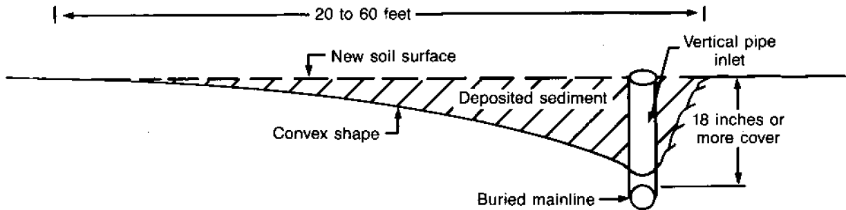
Fig. 2. An illustration of how the buried drain erosion and sediment loss control system corrects the convex end problem. Depth of cover is determined by including the sediment that will collect above the pipe.
