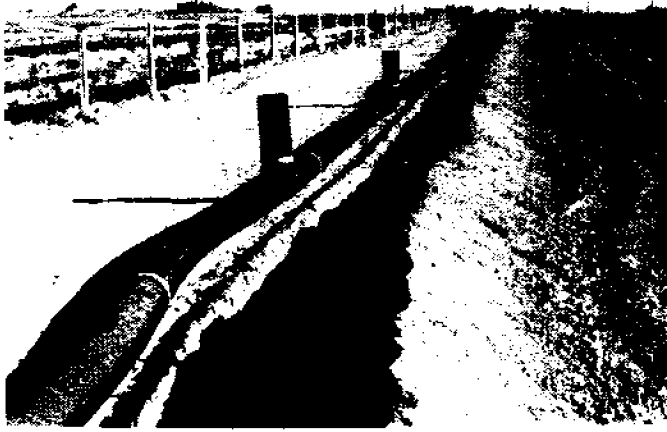
Fig. 5. A pipe with inlets connected ready to be placed in a trench made with a trenching machine.
