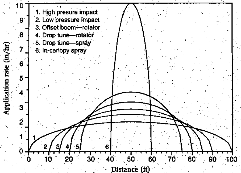
Figure 2. Comparison of relative application rates under various center pivot sprinkler packages.
