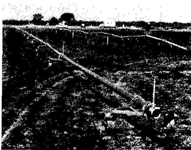
Pull-type wheel lateral system.
