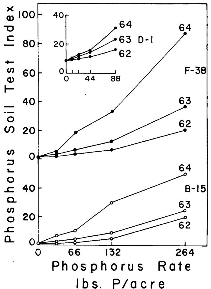
9. Effect of phosphorus fertilizer rate and year of application on soil test. Soils were sampled in late fall of 1964.
