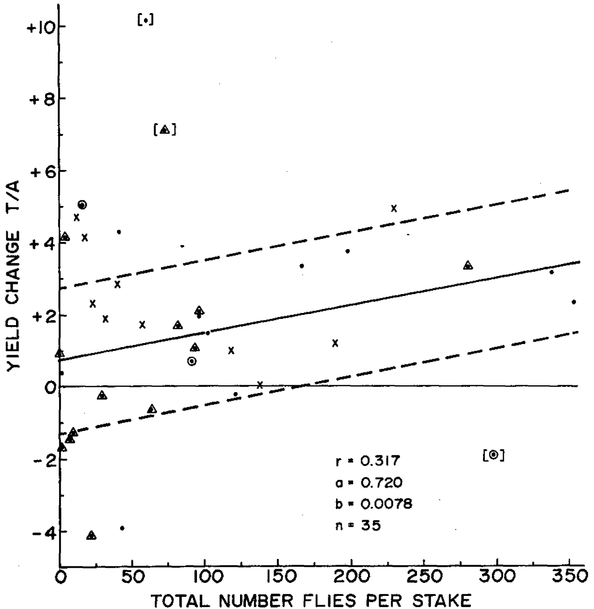
Figure 1.--The relationship between sugarbeet root maggot fly population and sugarbeet yield change in tons per acre following application of aldicarb at planting or soon after plant emergence. Year of observations: • 1974, △ 1975, X 1976, ⊙ 1977. Three data points in brackets are not included in regression. Dashed lines are \pm 2 tons per acre from regression line.
