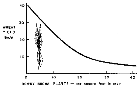
Fig. 1. Wheat yield of downy brome plants during U-1 tests at Tatonia test site.
