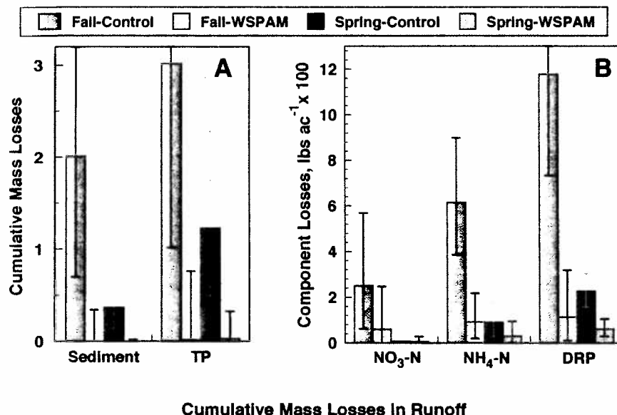
Fig. 1. Cumulative (A) sediment and TP and (B) nitrate-N, ammonium-N, and DRP mass losses in furrow runoff (Fall-Control, Fall-WSPAM) from the fall irrigation of late-summer manure-amended soils (Exp. 2) compared with that from an irrigation on the manure-amended soils (Spring-Control, Spring-WSPAM), which was delayed until the following spring (Exp. 3). All treatments were rototilled. Error bars represent 95% confidence limits on the treatment means.
